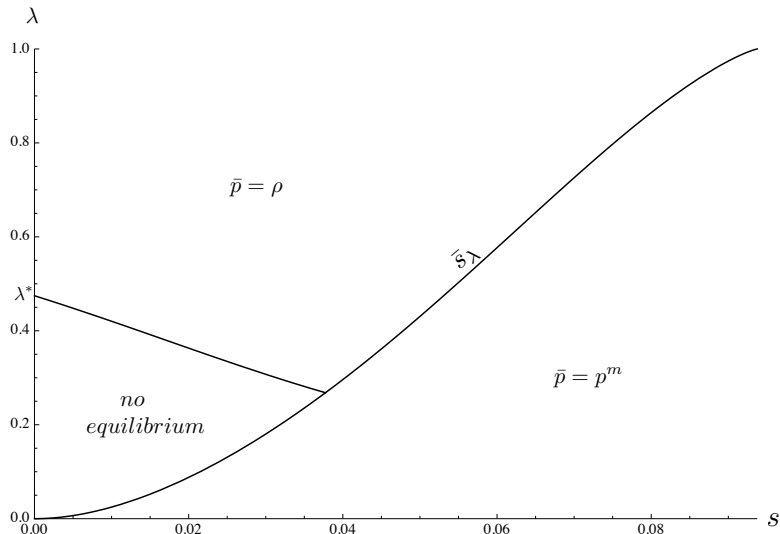
Figure 2: Different equilibrium cases depending on s and \lambda . Triangular area is where there is no equilibrium in the unobserved case.
