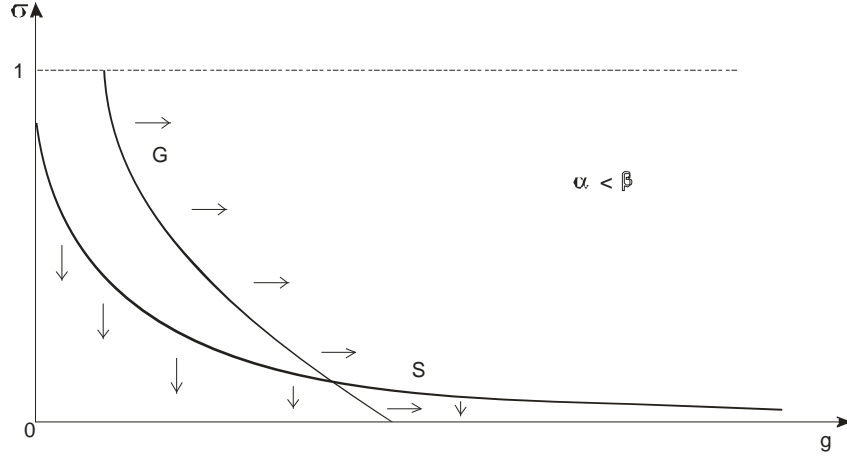
Figure 1. Effect of immigration on equilibrium public spending g and share of spending on transfers \sigma , for \alpha < \beta .
