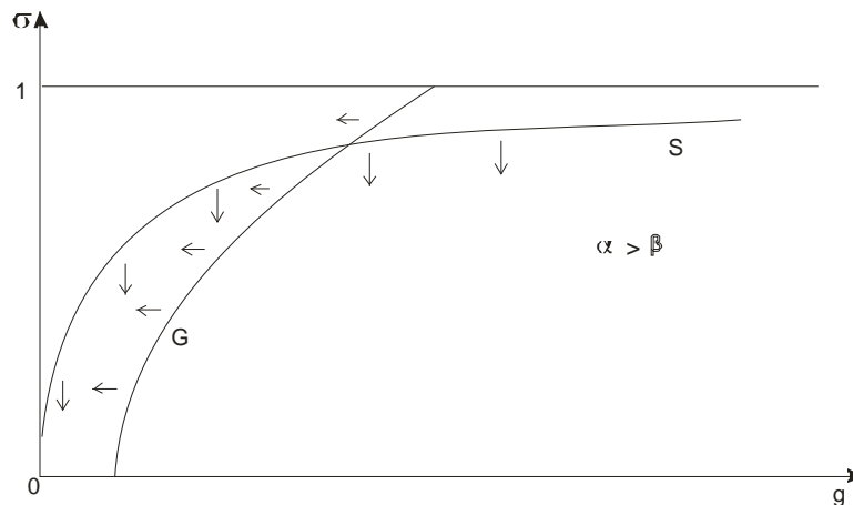
Figure 2. Effect of immigration on equilibrium public spending g and share of spending on transfers \sigma , for \alpha > \beta .
